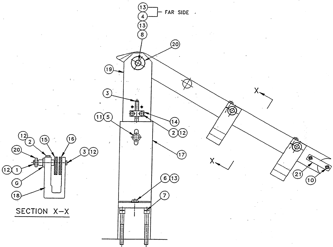
Figure 4. Upper Track Assembly
